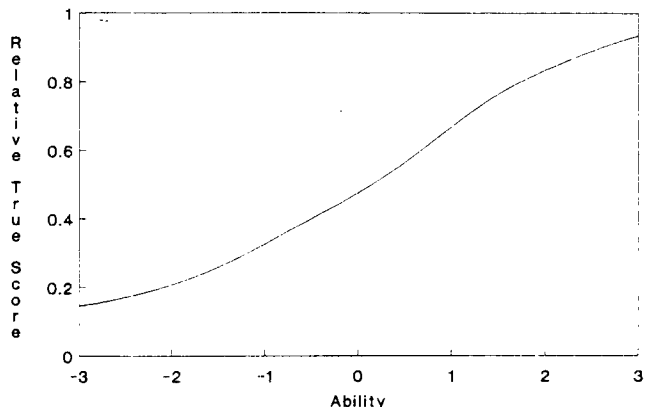
FIGURE 3. Relationship between ability and true score
